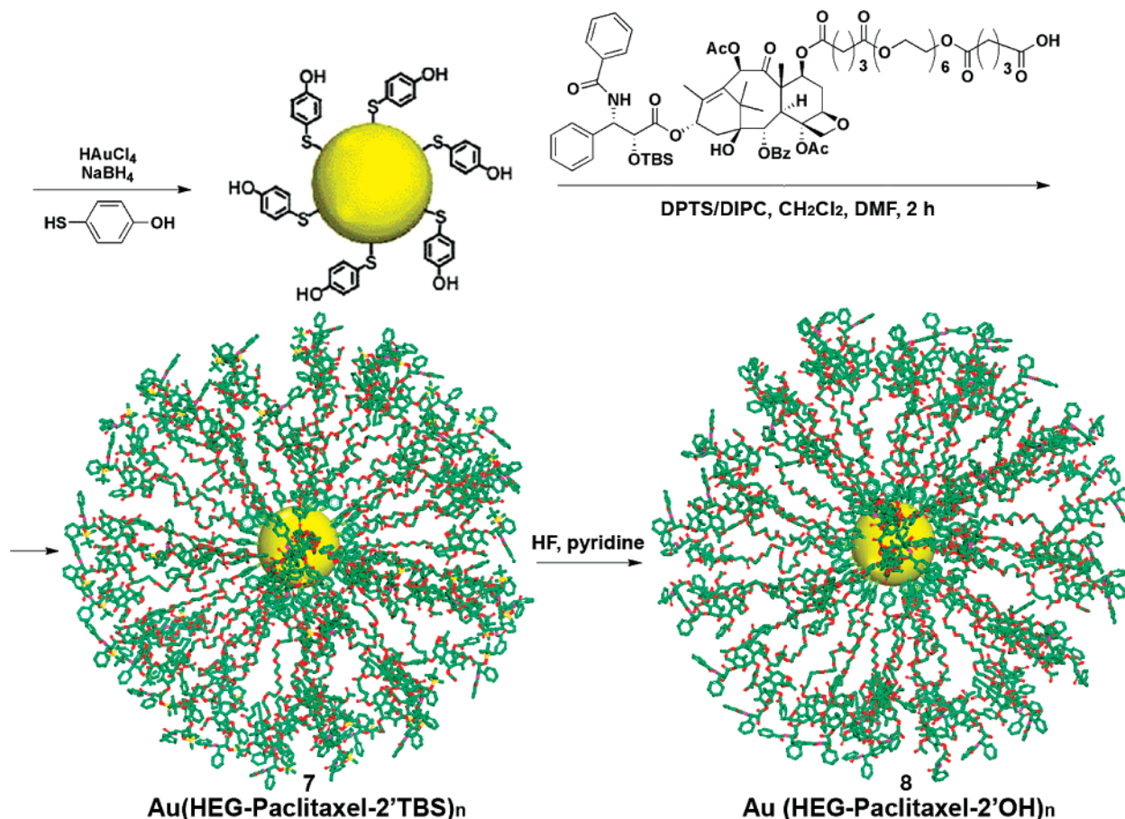
Scheme 2. Covalent Coupling of Paclitaxel to 4-Mercaptophenol-Modified 2 nm Gold Nanoparticles
