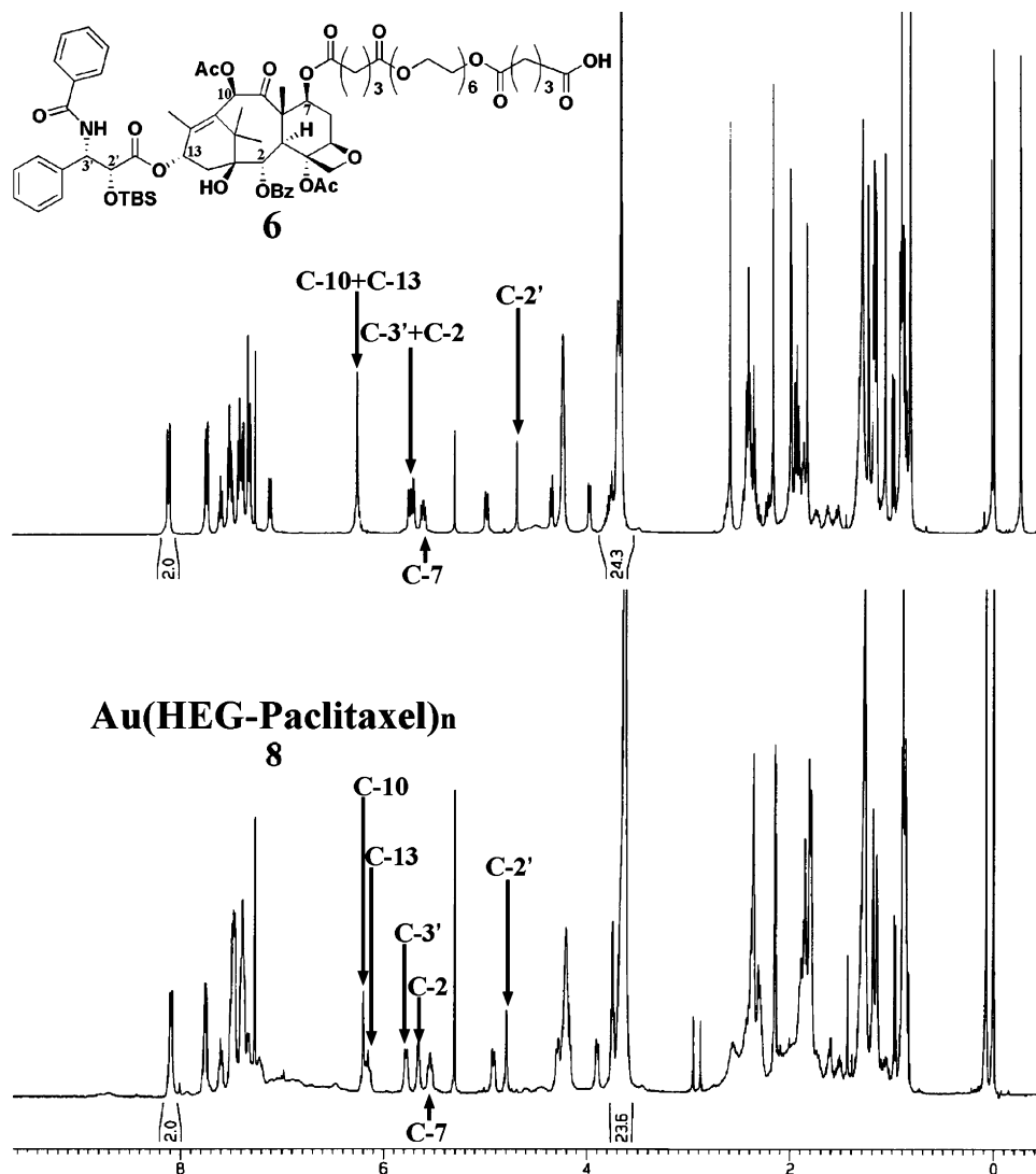
Figure 2. ^1\text{H} NMR spectra of paclitaxel analogue 6 (top) and the isolated hybrid structure 8 (bottom).
